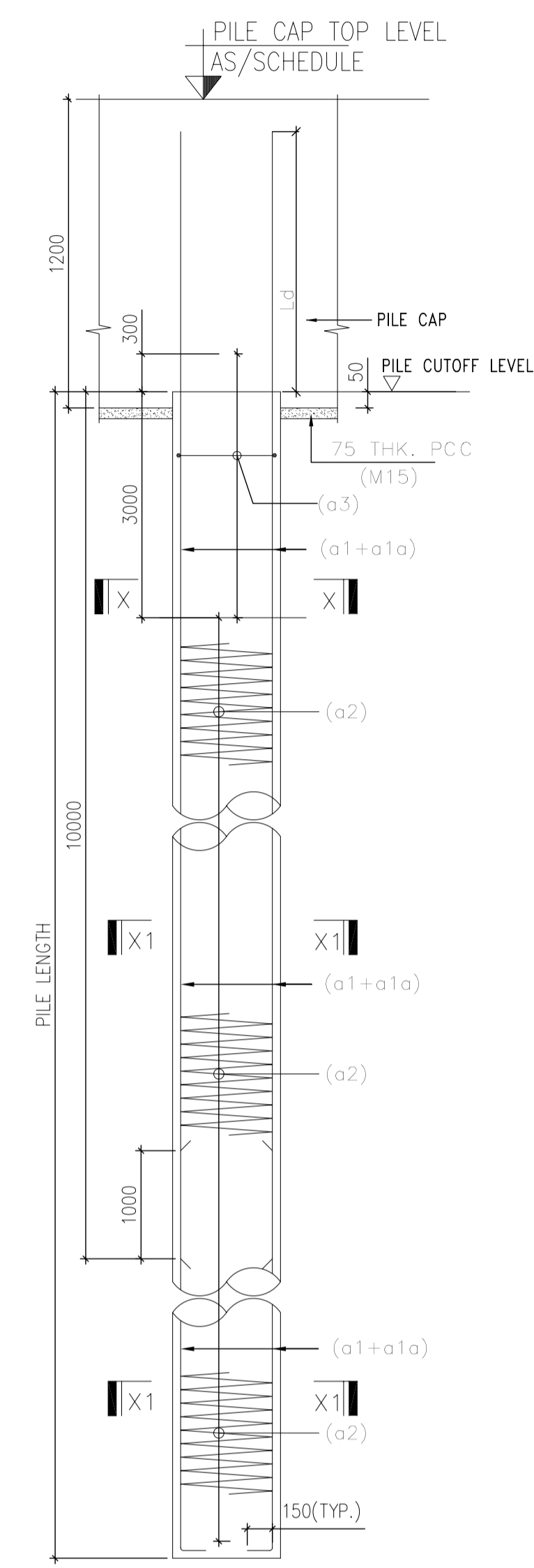
DETAIL OF PILE PC1, PC2 & PC3 SCALE 1:50 PILE REINFORCEMENT SCHEDULE
