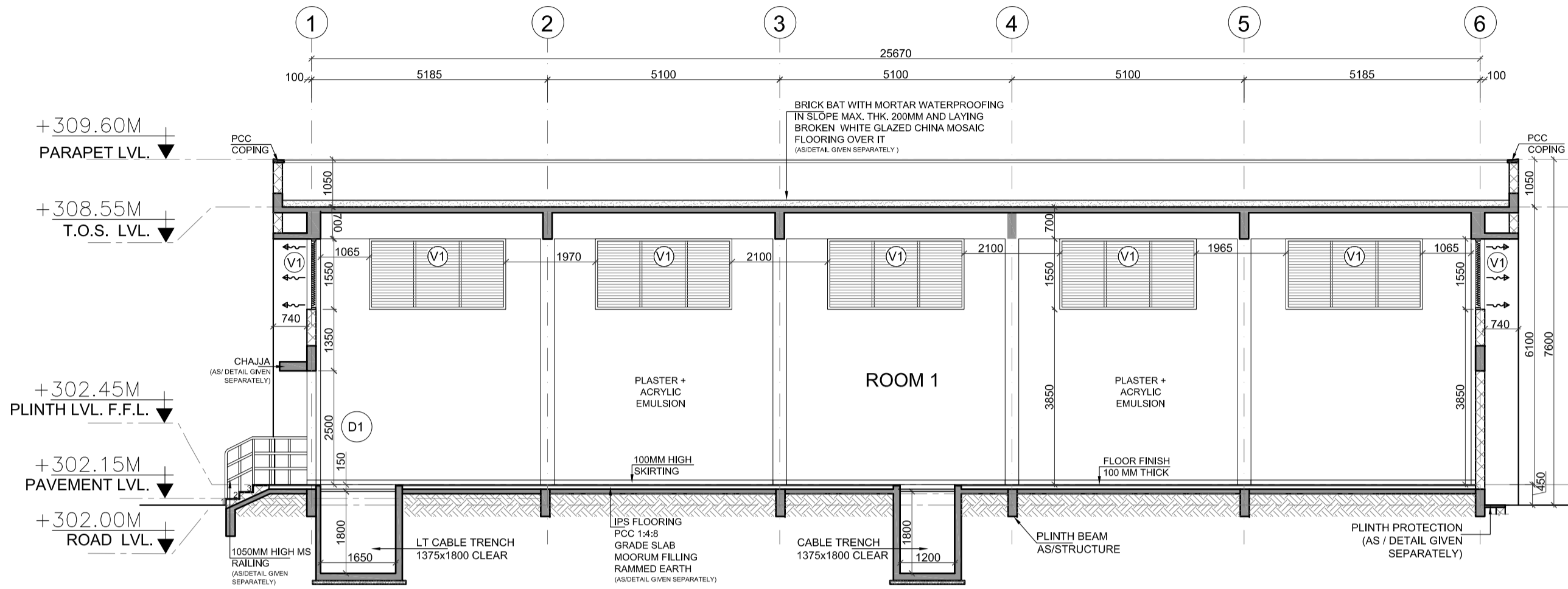
SECTION AA
