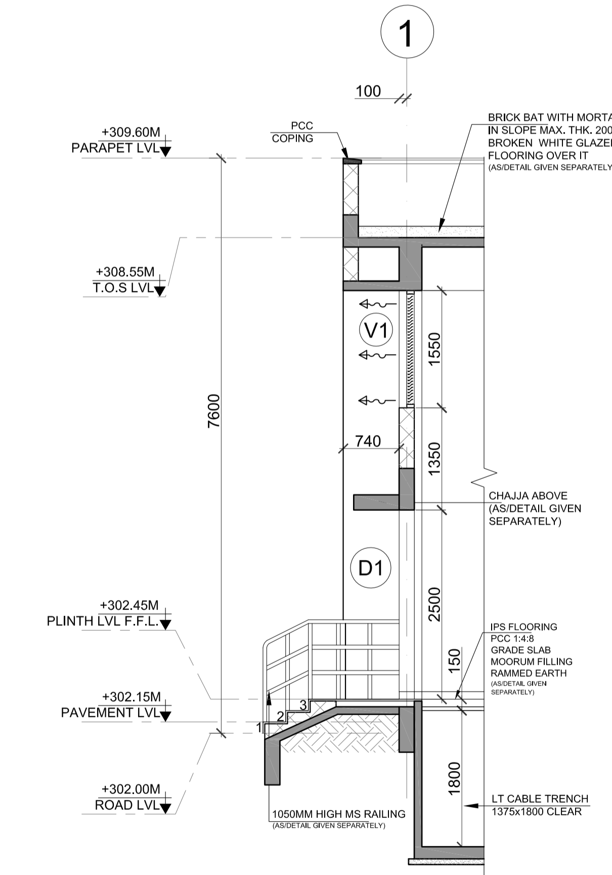
WALL SECTION - 2
