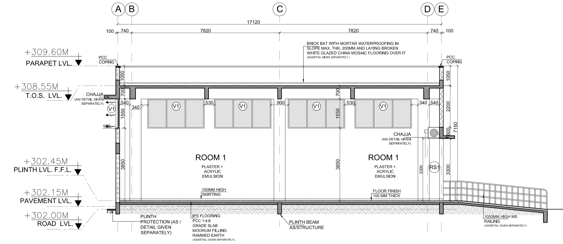
SECTION BB
