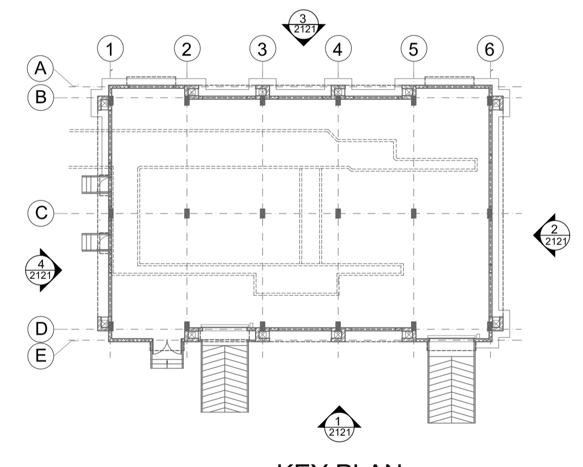
KEY PLAN SCALE 1:250
